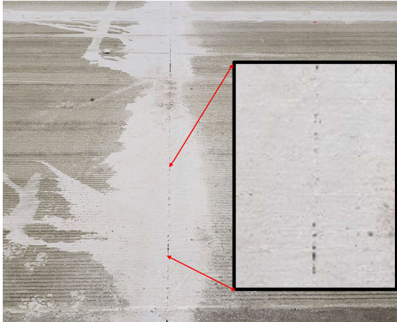
Figure 3 Photo of Dried Slurry After Narrow/Contraction Joint Sawing
